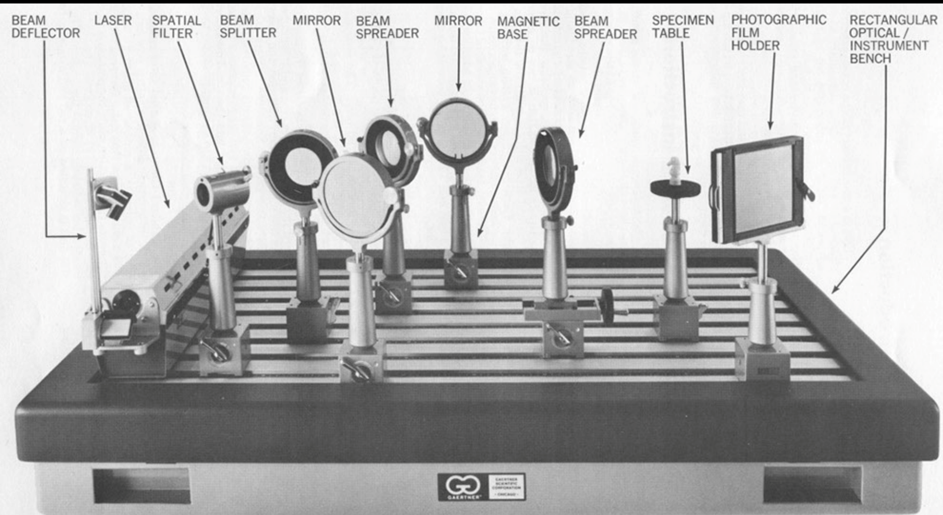
GAERTNER-JEONG HOLOGRAPHY SYSTEM
